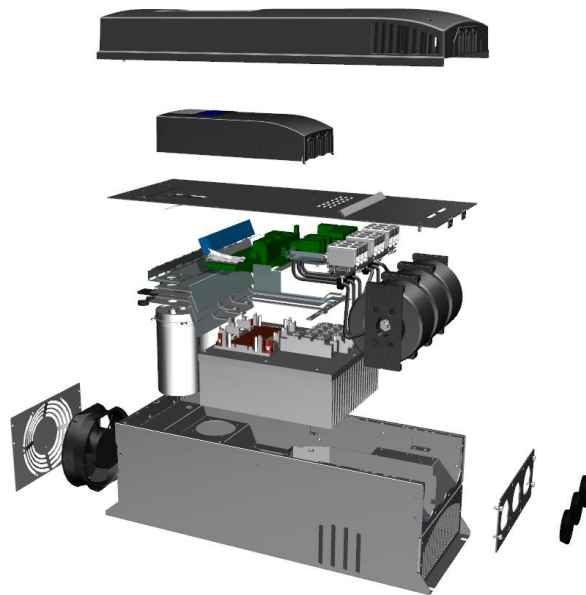
Figure 1: The exploded illustration of the drive with its main components.
