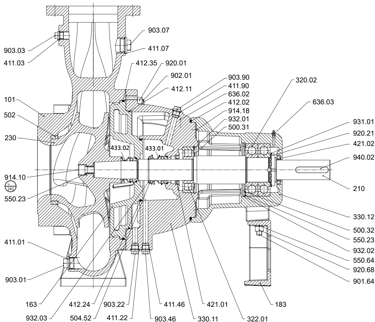
Fig. 9: Sewatec with bearing brackets S05 to S08
