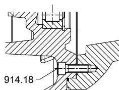
Fig. 12: Detail X
