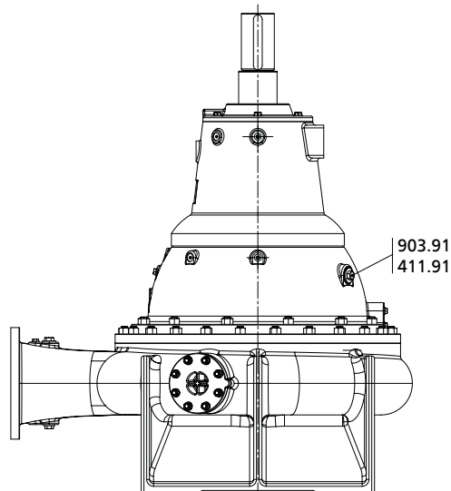
Fig. 23: Drilled hole required during manufacturing, bearing brackets S09 and S10
