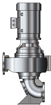
Fig. 4: Sewabloc - vertical (V): Pump set with directly flanged motor (B5/V1 type of construction), with base suction elbow
