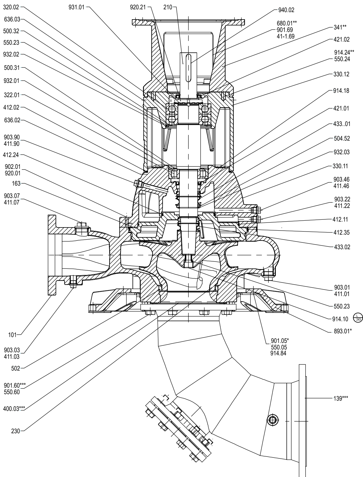
Fig. 10: Sewatec with E impeller – pump for underfloor installation and installation with universal-joint shaft
