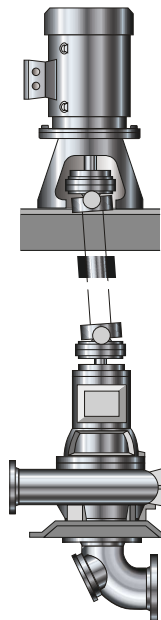
Fig. 7: Sewatec - vertical (VGW): Pump set with soleplate for pump and motor, support frame, drive lantern, suction elbow and universal-joint shaft
