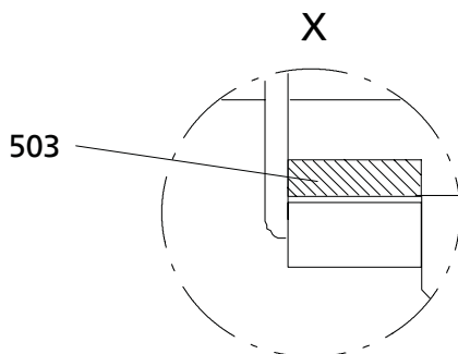
Fig. 16: Detail X: impeller wear ring for K impeller
