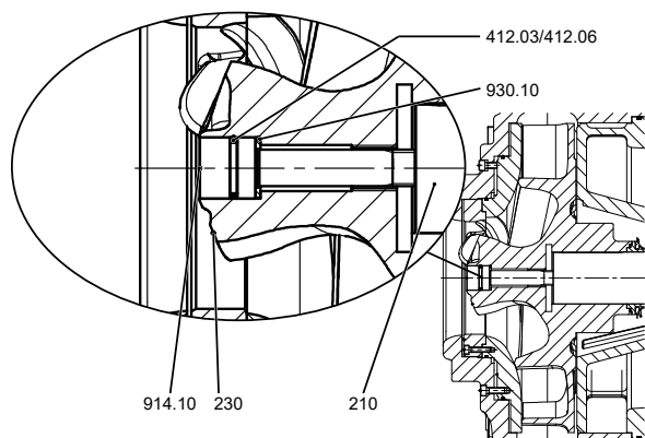
Fig. 20: Impeller fastening for bearing bracket S07 (impeller type D)
