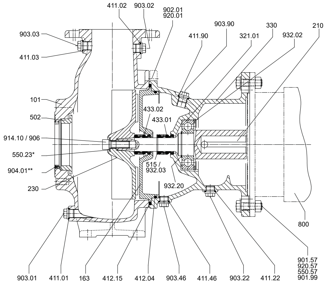
Fig. 13: General assembly drawing of Sewabloc; * if any, ** only for sizes 100-253, 100-254, K 100-316
