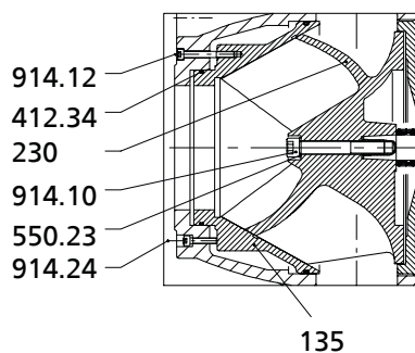
Fig. 17: D impeller (single-vane impeller)
