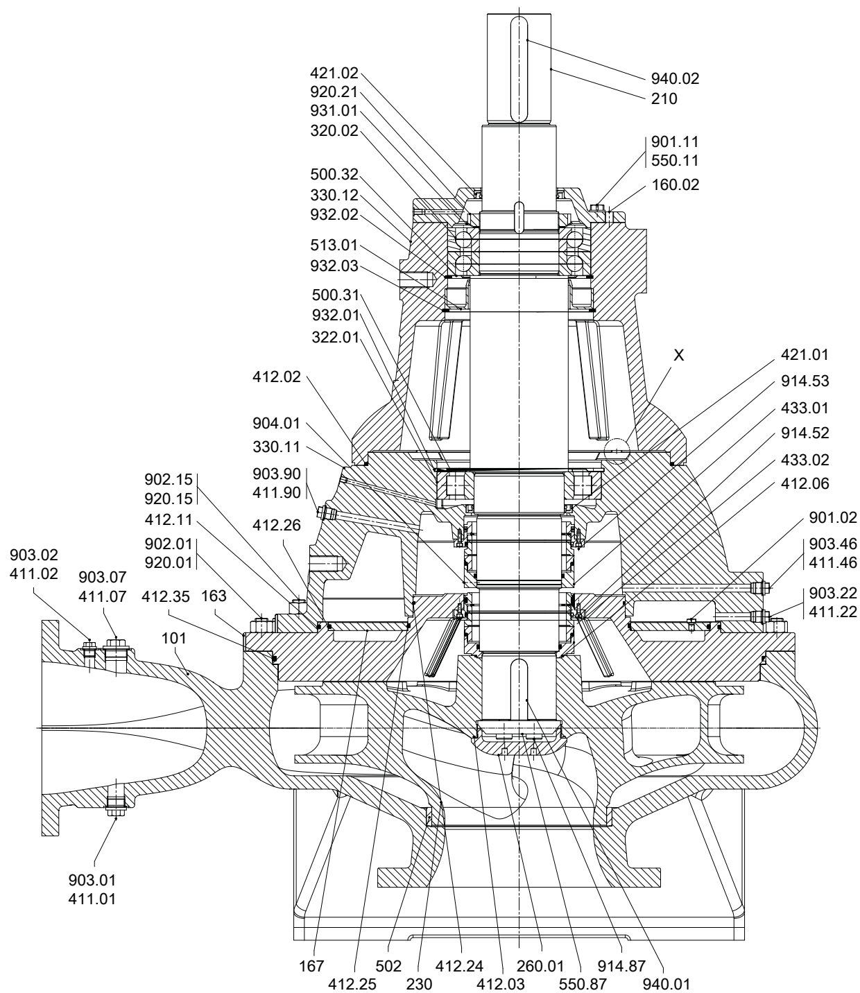
Fig. 11: Sewatec with bearing brackets S09, S10
