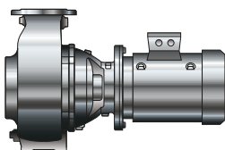
Fig. 3: Sewabloc: Pump set with directly flanged motor, C-face configuration, horizontal installation
