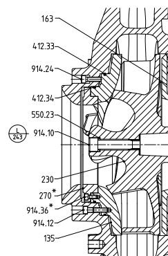
Fig. 18: D impeller (multi-vane impeller)
