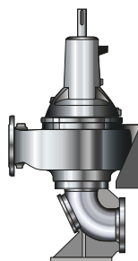
Fig. 5: Sewatec - vertical (V): a) Pump set on suction elbow b) Pump set on concrete base
