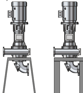
Fig. 6: Sewatec - vertical (VU): a) Pump set, C-face configuration, with motor pedestal, drive lantern, coupling, coupling guard and suction elbow, b) Pump set with soleplate, drive lantern, coupling, coupling guard and suction elbow
