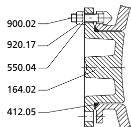
Fig. 21: Inspection hole, bearing brackets S01 to S08
