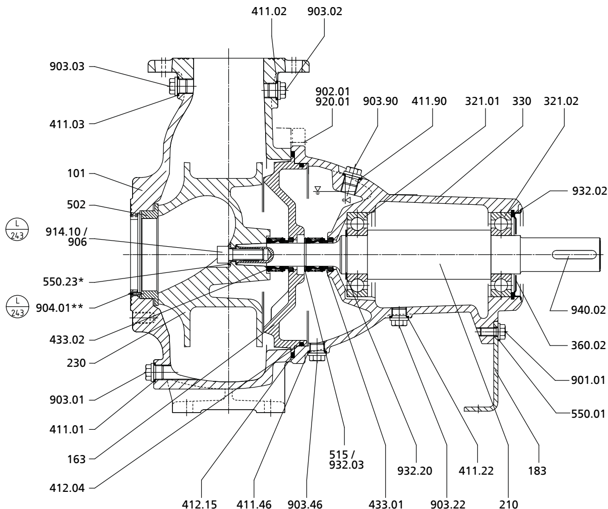
Fig. 8: General assembly drawing of Sewatec - with bearing brackets S01, S02, S03, S04, impeller type E; * if any, ** only for sizes E 100-250, E 100-253, E 100-317, E 150-317, K 100-253, K 100-254, K 100-316
