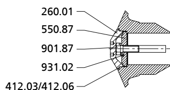
Fig. 19: Impeller fastening for bearing brackets S07 and S08 (impeller types E and K), except Sewatec size 500-632
