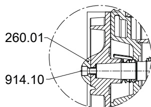
III. 18: Roue F
