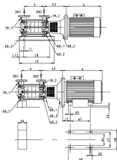
Fig. 5: Multitec E dimensions
