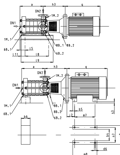
Fig. 6: Multitec F dimensions
