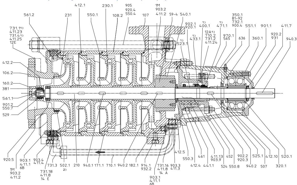
Fig. 8: Multitec, installation type A, size 65-100
