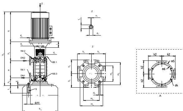
Fig. 7: Dimensions of Multitec V / Multitec-RO
