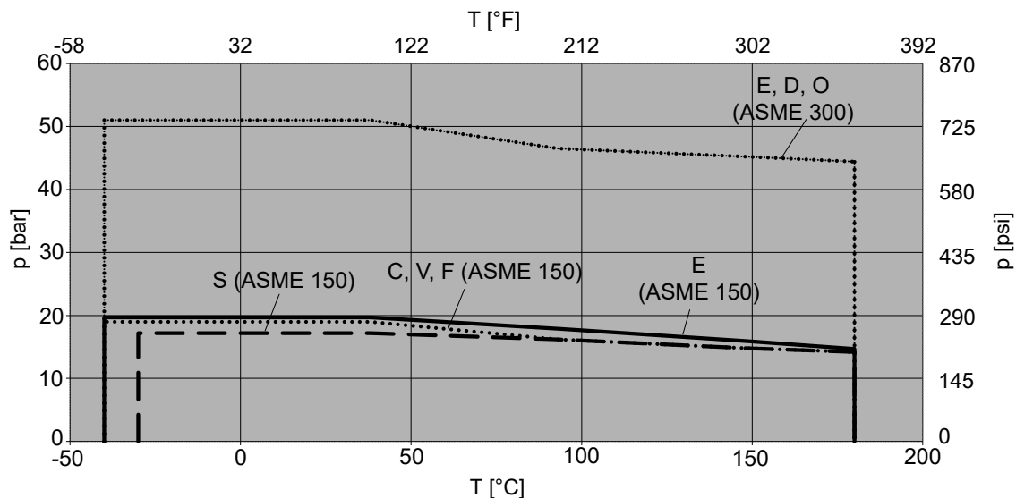
Fig. 4: Pressure limits and temperature limits of ASME flanges for versions with bearing bracket CA (complementary sizes)
