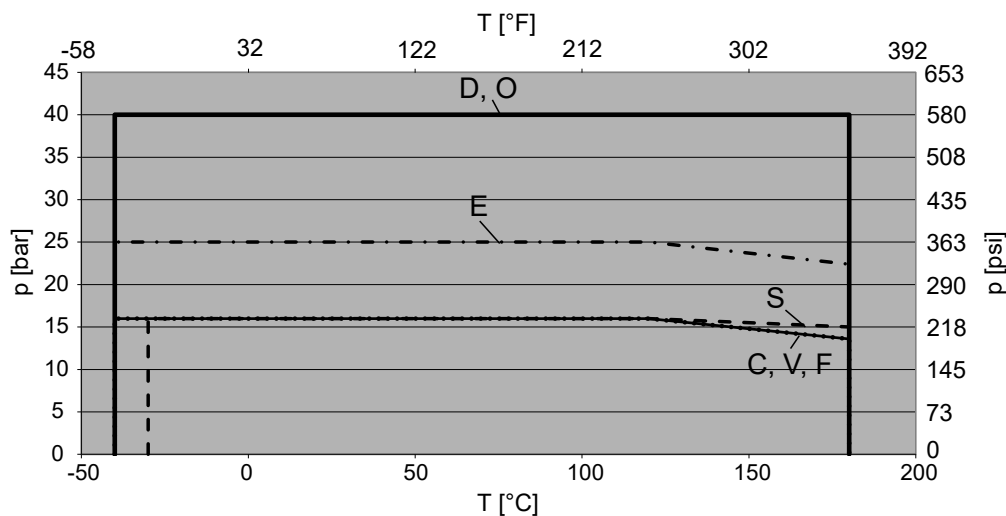
Fig. 2: Pressure limits and temperature limits of the pump for versions with bearing bracket CA (complementary sizes)
