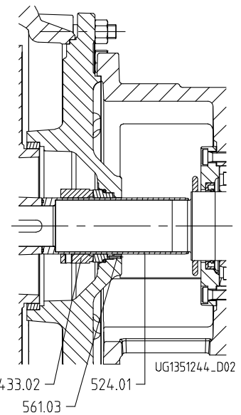
Version with labyrinth seal
