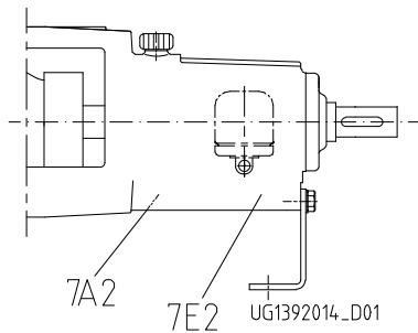
Fig. 8: Connections for version with coolable bearing bracket
