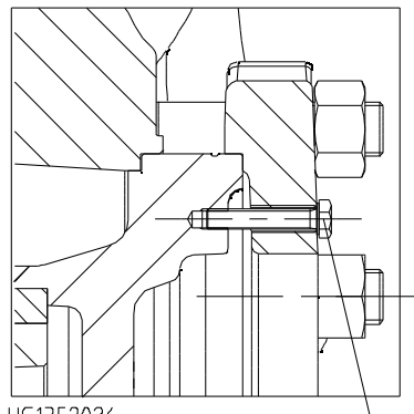
Version with clamped casing cover
