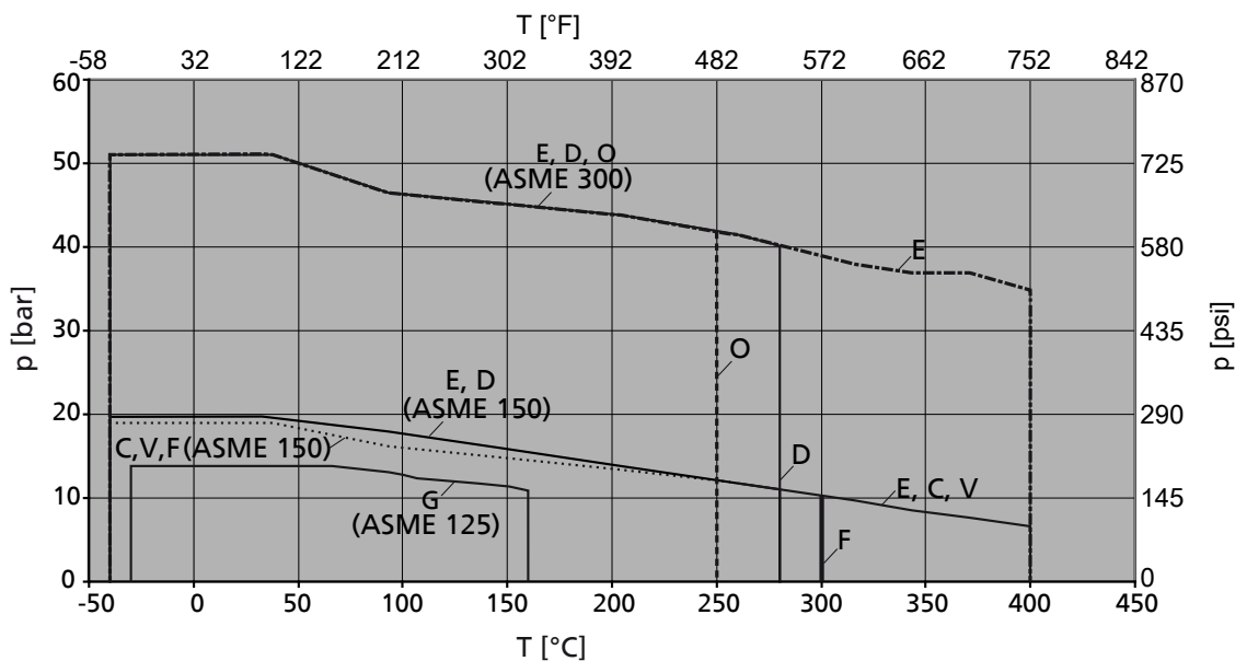
Fig. 3: Pressure limits and temperature limits of ASME flanges with bearing bracket CS
