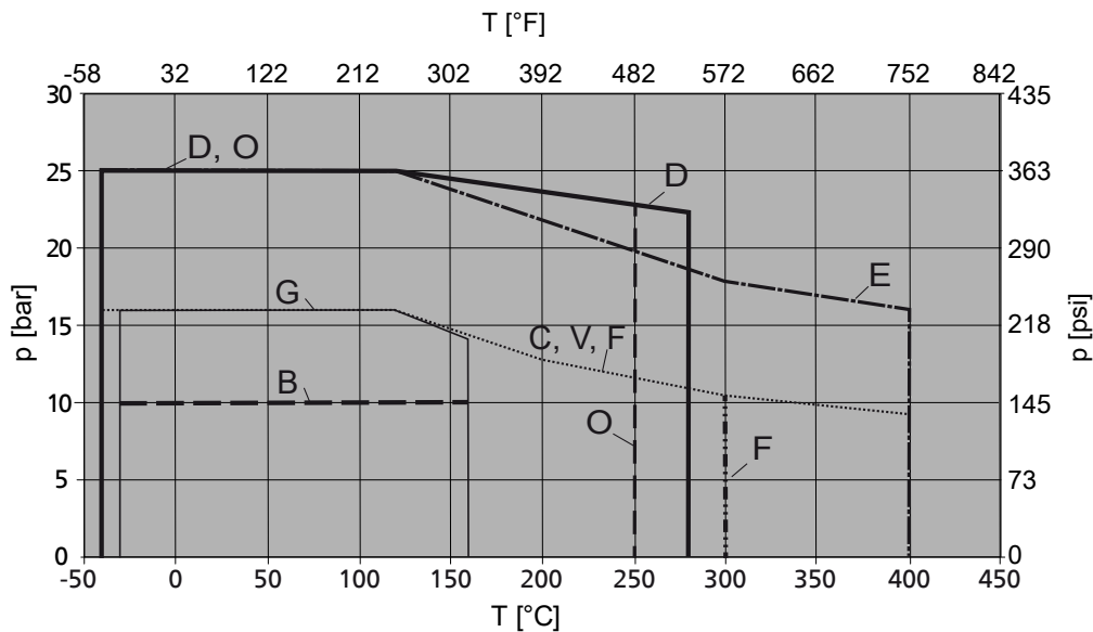
Fig. 1: Pressure limits and temperature limits of the pump with bearing bracket CS
