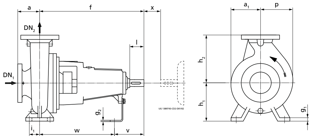
III. 1: Dimensions pompe
