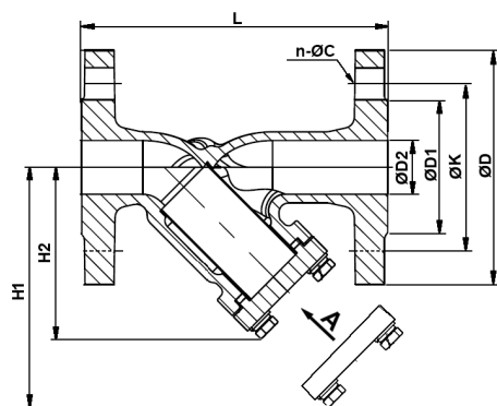
DN15-32
