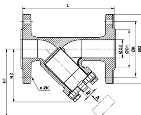
DN40
