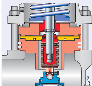
Balanced piston design K10
