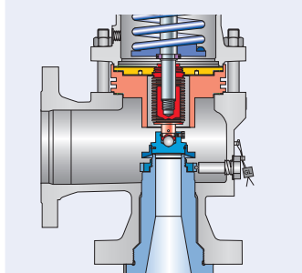
Inconel bellows J83
