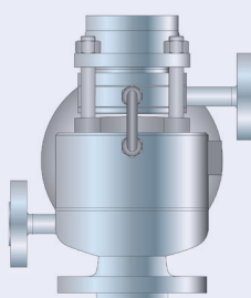
Balanced piston design K10
