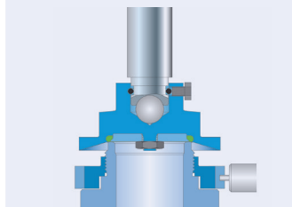
O-ring disc J21: CR "K" J22: EPDM "D" J23: FKM "L" J20: FFKM "C"
