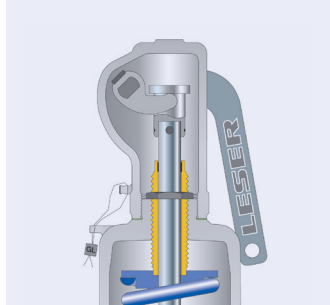
Lift indicator J39: Adaptor for lift indicator H4 J93: Lift indicator
