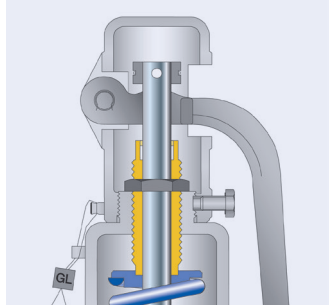
Bolted cap H1 K01
