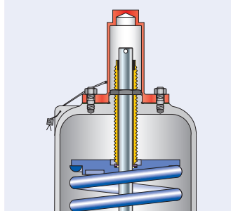
O-ring disc J21: CR "K" J22: EPDM "D" J23: FKM "L" J20: FFKM "C"
