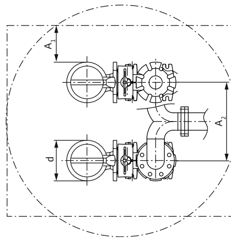
Fig. 3: Distances minimales
